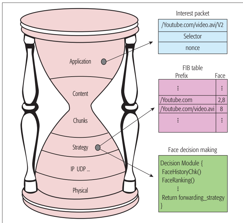
Figure 1. NDN network stack model.
