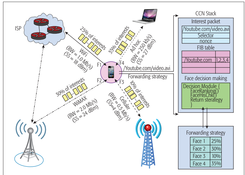
Figure 3. Leveraging the multiple communication interfaces in an IC-MCN.
