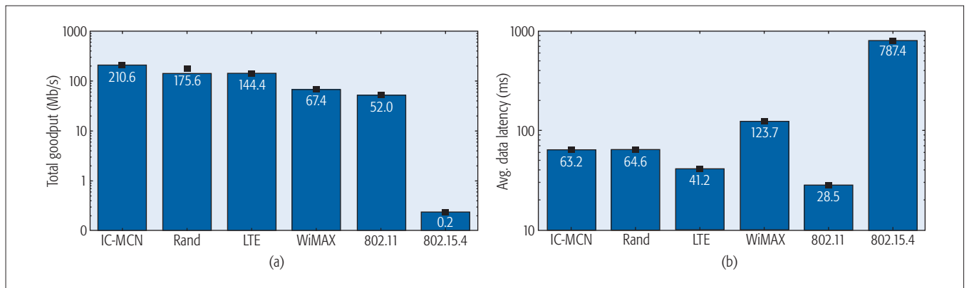
Figure 4. Achieved a) goodput; b) latency measurements for each forwarding strategy. We observe that weighing interfaces based on observations (IC-MCN) allows higher goodput and lower latency to be achieved than simple randomized load balancing (Rand).
