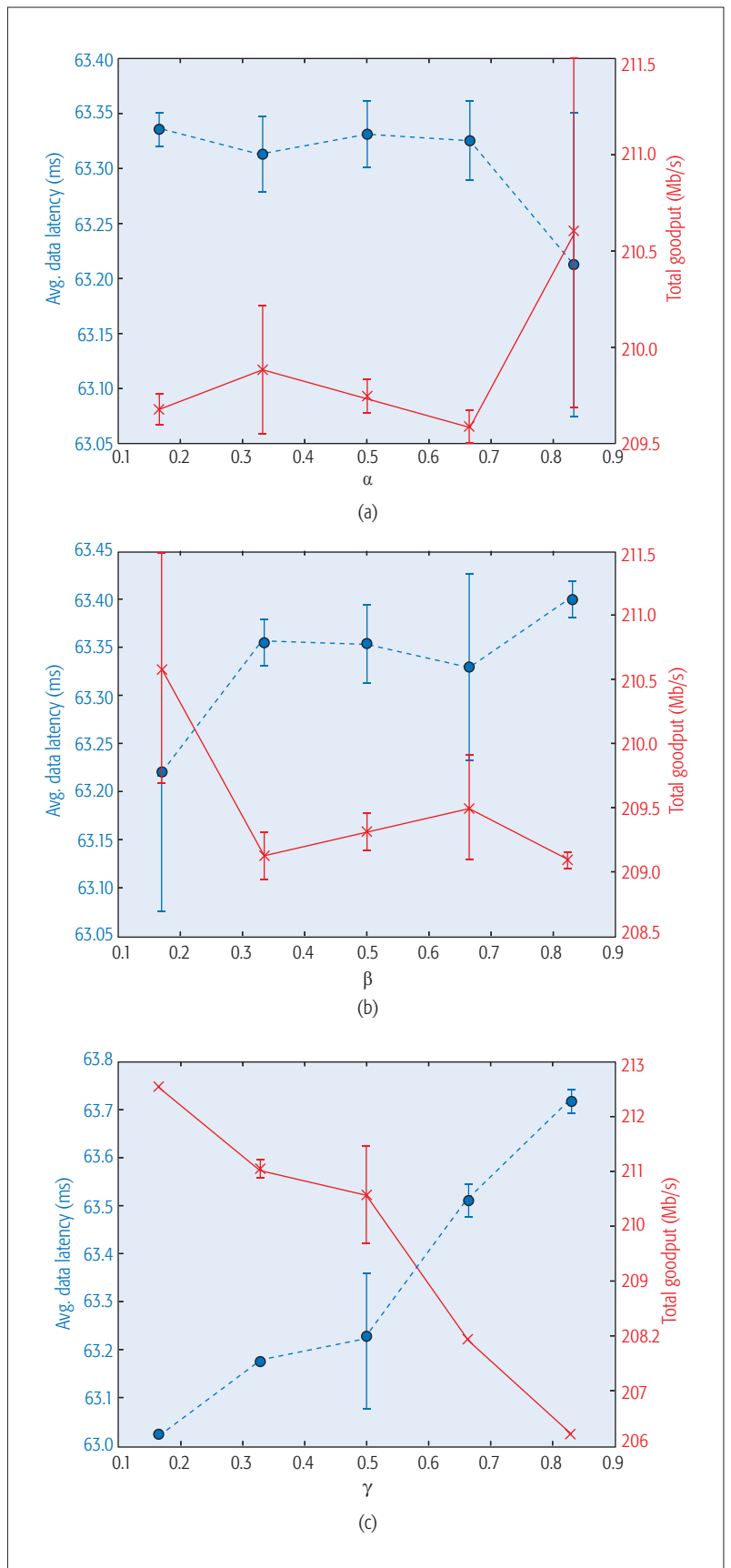
Figure 5. Effects of configuration parameters on latency and goodput. In each plot, we vary one parameter over {0.167, 0.333, 0.500, 0.666, 0.833} and fix the others at their default values ( \alpha = 0.833 , \beta = 0.167 , \gamma = 0.500 ). Latency is given by the blue dashed line and the left y-axis; goodput is given by the red solid line and the right y-axis.
